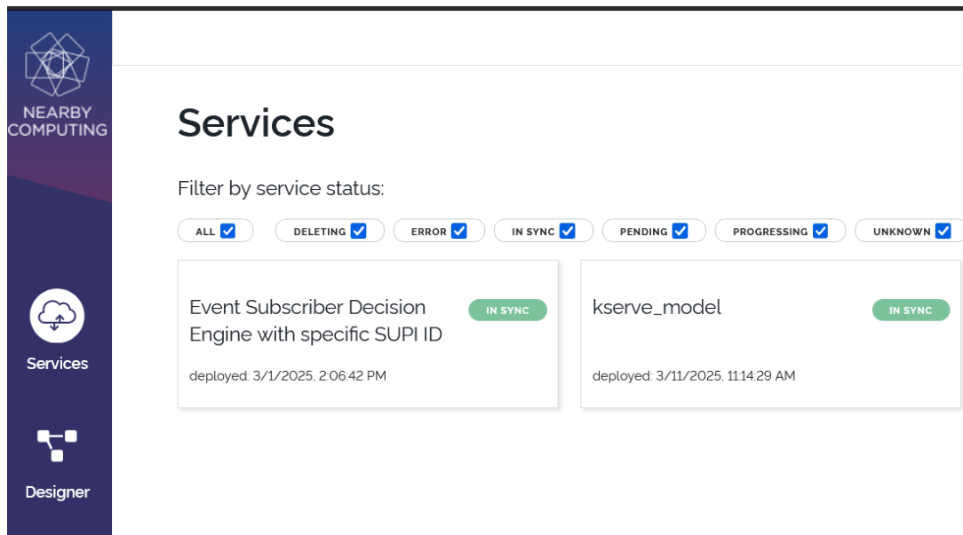
Figure 31: Service monitoring through NearbyOne
