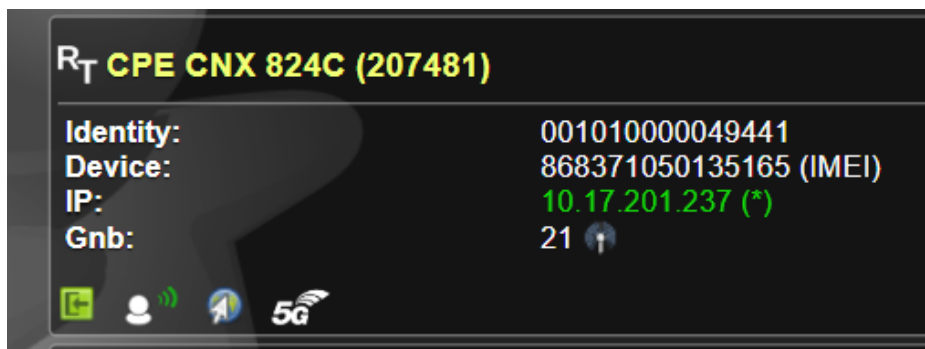
Figure 39: Iperf node 8
