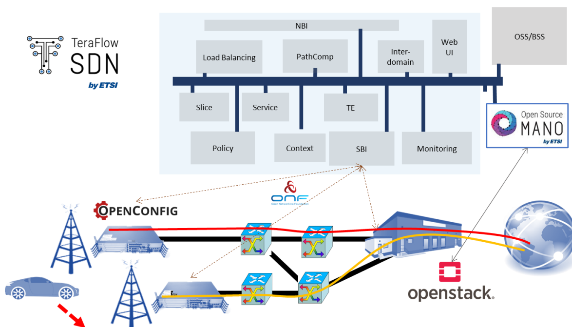
Figure 11 Proposed architecture for Over-the-air vehicular software updates with robust V2X connectivity
