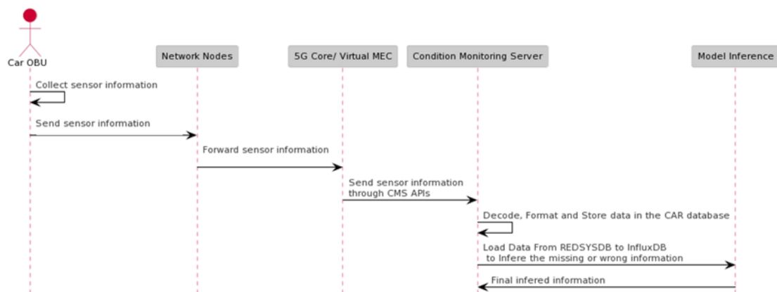
Figure 27 Sequence diagram for vehicular condition monitoring with efficient computation
