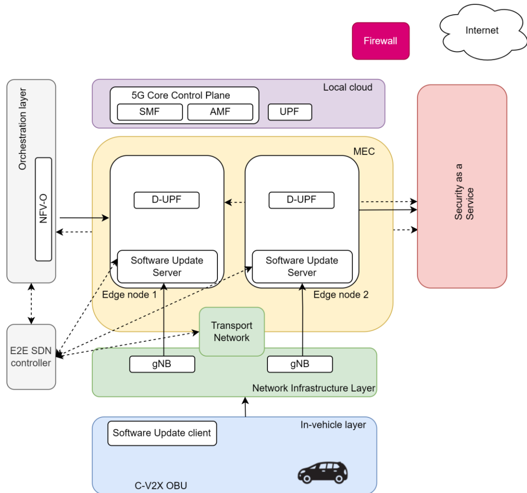
Figure 3 System architecture for over-the-air software updates
