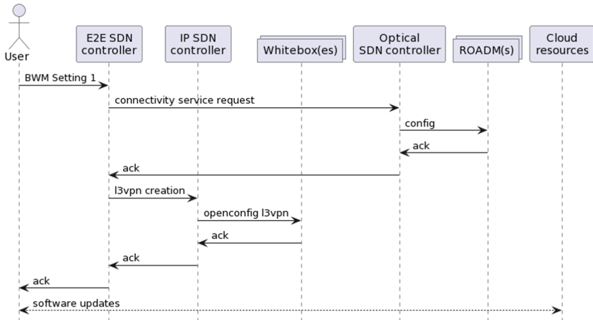
Figure 28 Sequence diagram for over-the-air vehicular software updates with efficient computation
